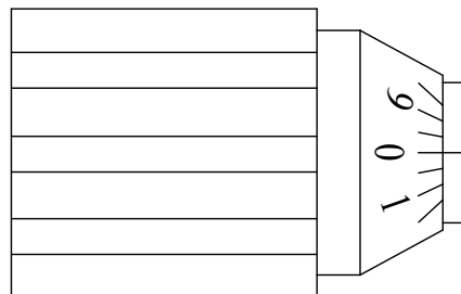
Fig. 7: 1 revolution = 100 % stroke length
