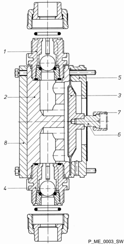
Fig. 5: Cross-section through the liquid end
